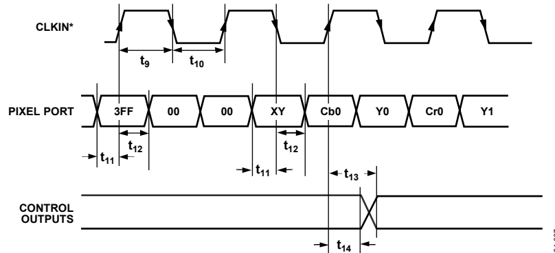
Figure 7. ED/HD-DDR Input, 8-/10-Bit 4:2:2 YCrCb (EAV/SAV), Input Mode 010
